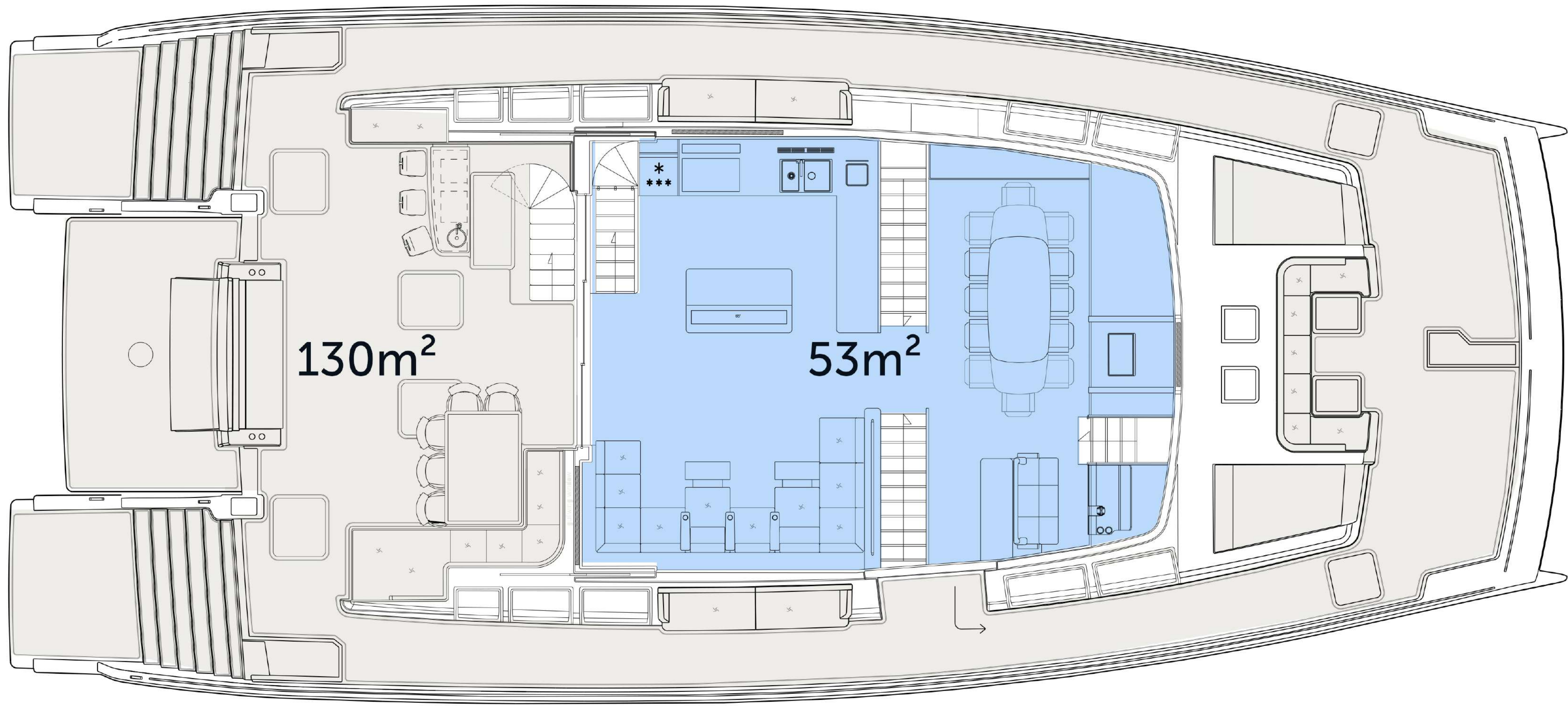
Main deck
