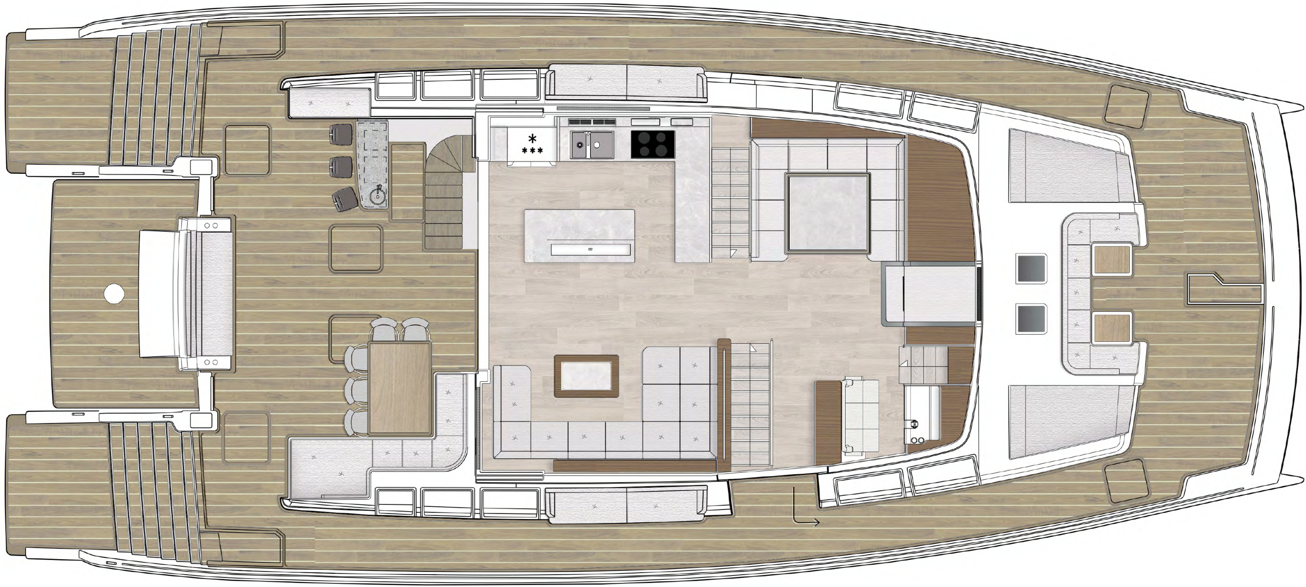
Main deck
