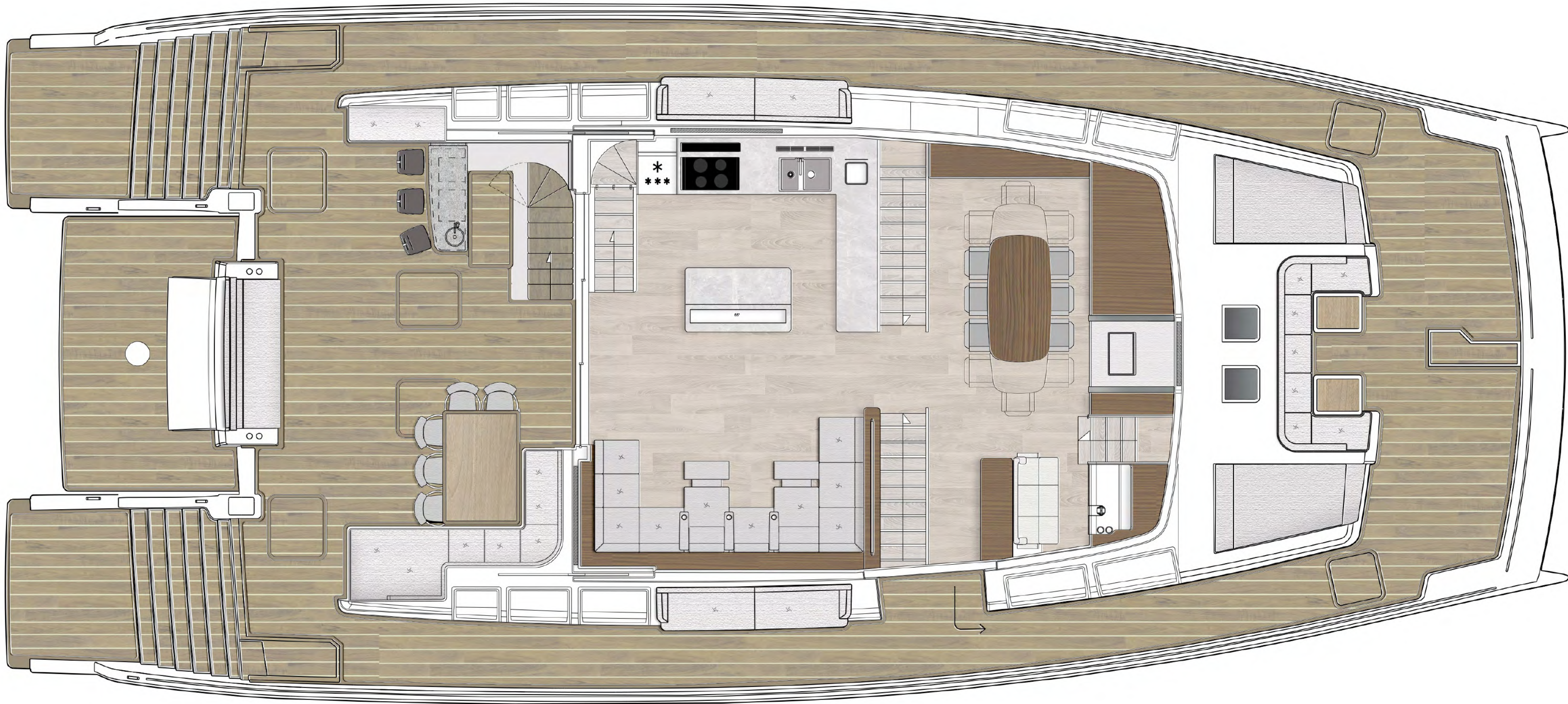
Main deck
